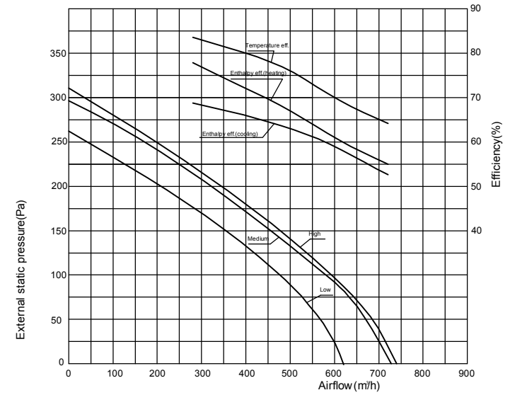
XHBQ-D6TH Performance Chart
