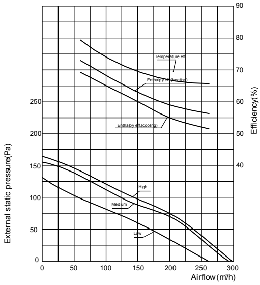
XHBQ-D2TH Performance Chart
