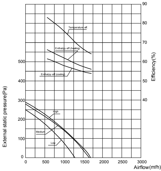
XHBQ-D13TH Performance Chart
