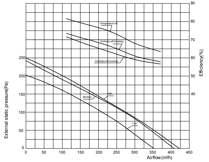
XHBQ-D3TH Performance Chart
