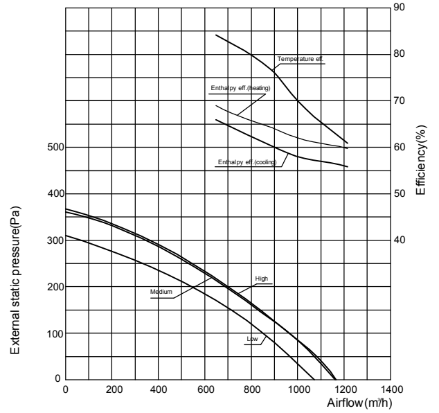
XHBQ-D10TH Performance Chart
