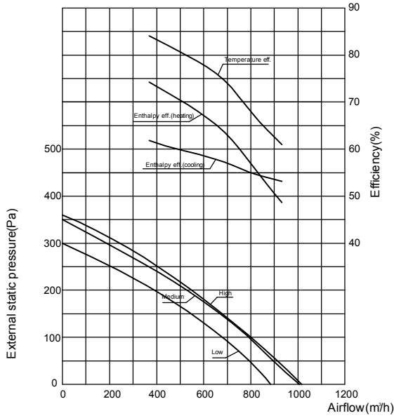
XHBQ-D8TH Performance Chart
