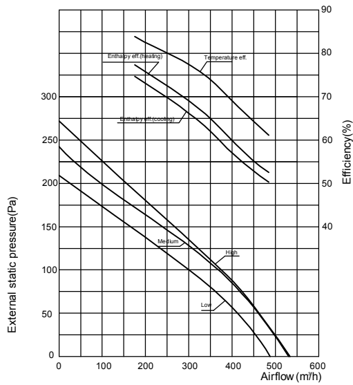
XHBQ-D4TH Performance Chart
