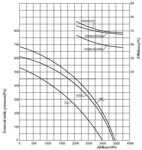
XHBQ-D30TG Performance Chart
