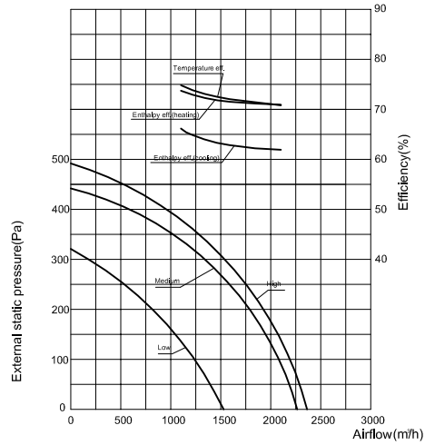
XHBQ-D20TG Performance Chart
