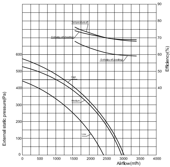
XHBQ-D25TG Performance Chart
