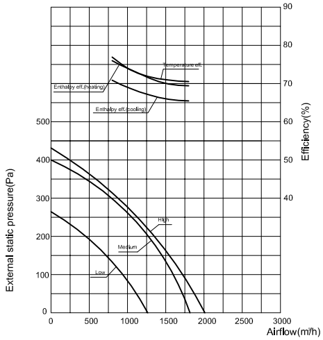
XHBQ-D15TG Performance Chart
