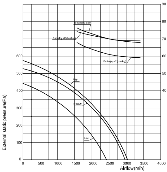
XHBQ-D25TG Performance Chart
